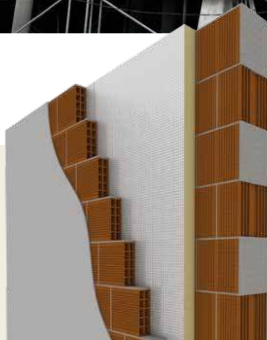
Ventilated facade with FIBRANgeo B-570-YM
