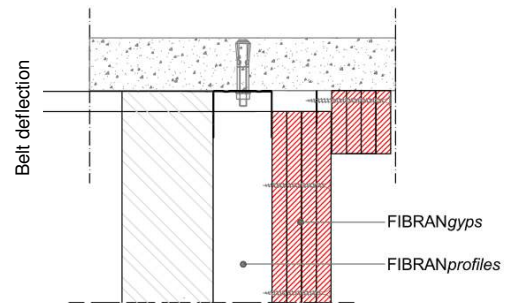
Detail. 4 DESOLIDARIZATION FLOOR - WALL
