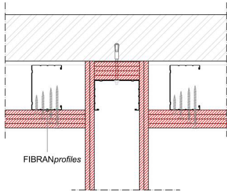
Detail. 1 FITTING WITH FIRE RESISTANT WALL
