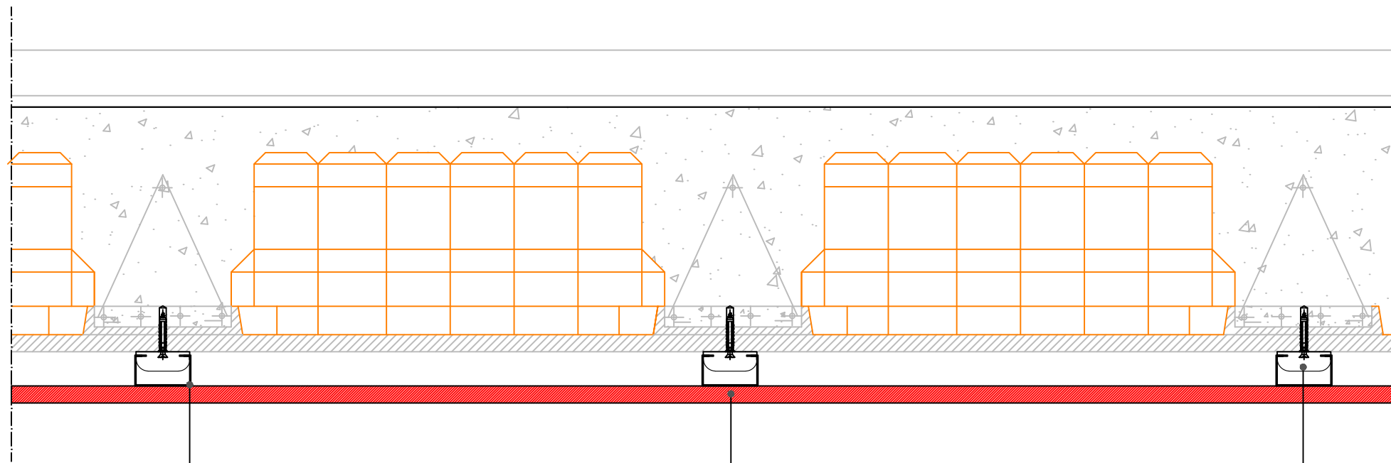
FIBRAN profiles MONTANTE 4927
