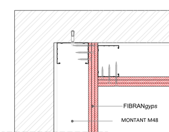
Part. 2 Joint d'angle
